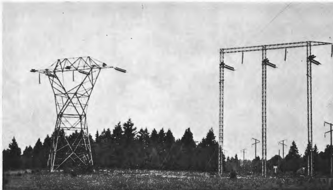
New light weight angle tower construction (right) saves steel.
