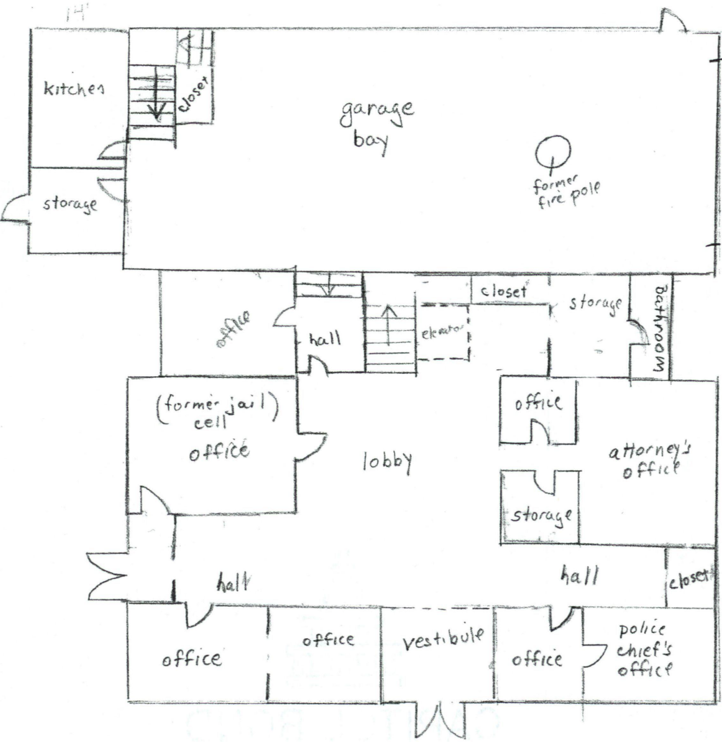
MOREHEAD CITY MUNICIPAL BUILDING FIRST FLOOR PLAN NOT TO SCALE
