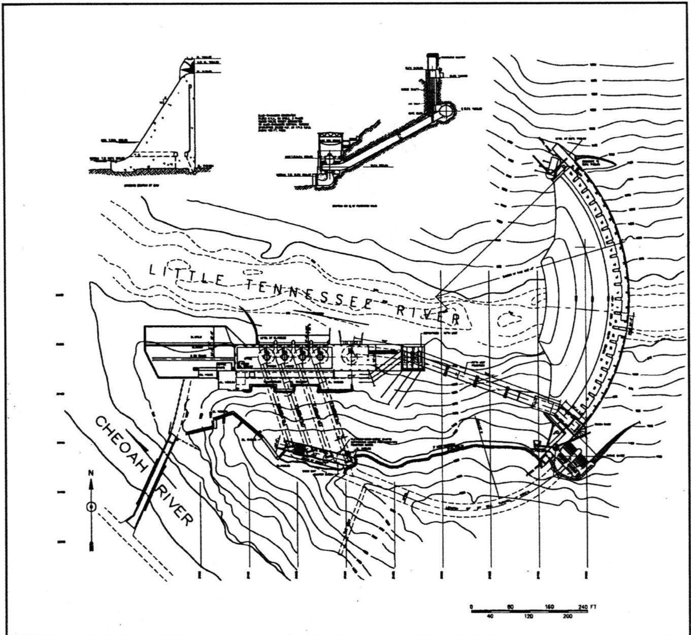
Figure No. 1. Cheoah Hydroelectric Development general plan.
