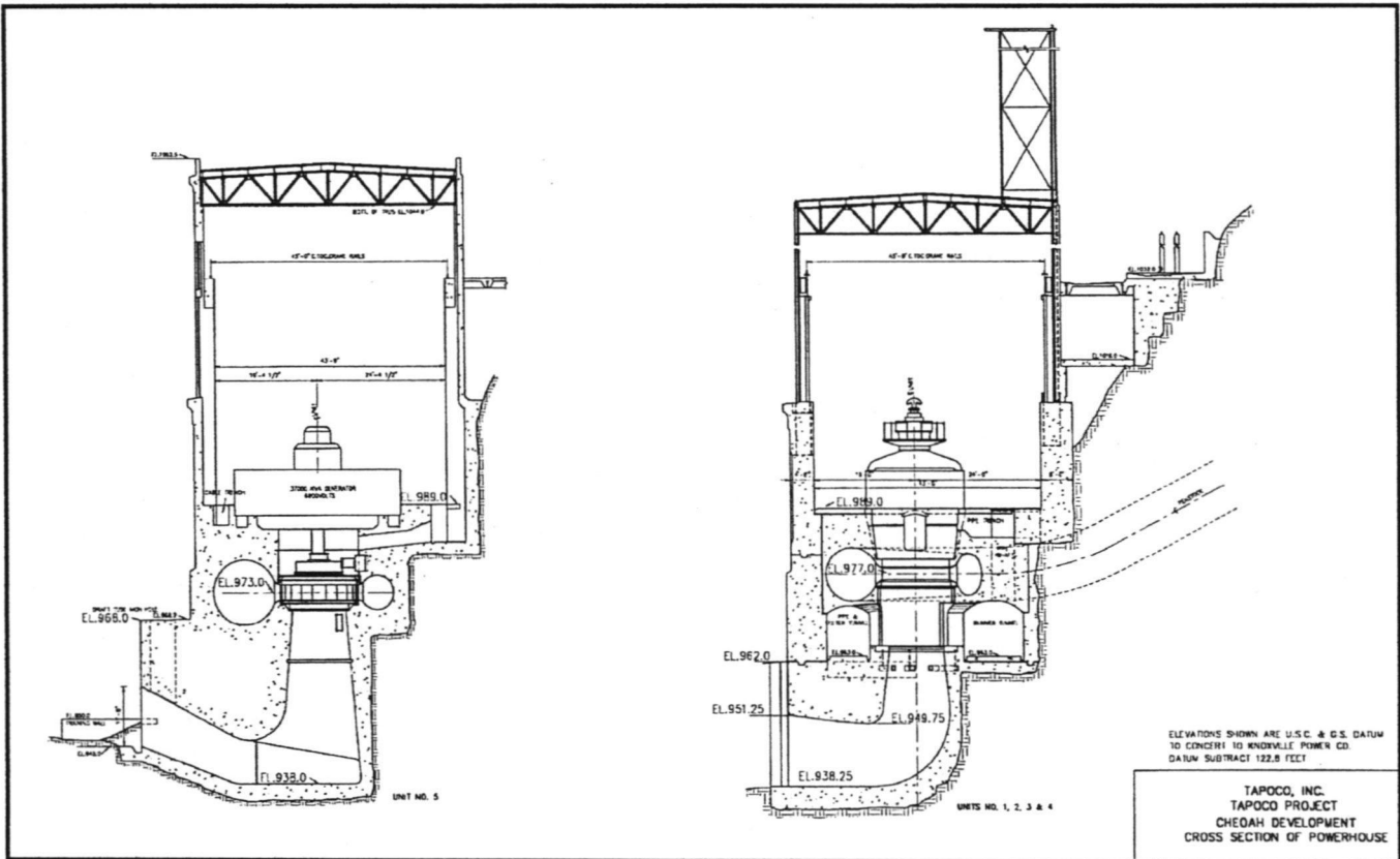
Figure No. 2. The Cheoah Hydroelectric Development, cross section of powerhouse.
