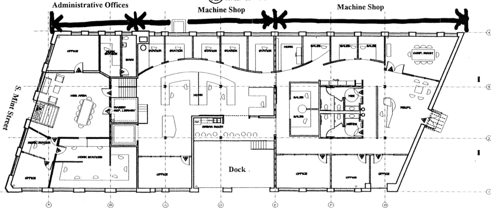
1 FIRST FLOOR PLAN AU SCALE: 1/8" = 1'-0"
