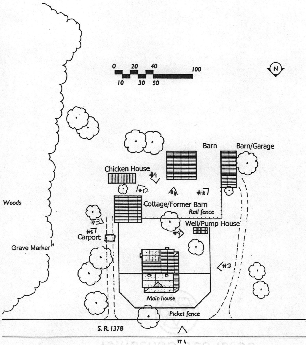
Jesse W. and Lillian F. Penny House and Outbuildings Site Plan (Drawing by Robin J. Stancil)
