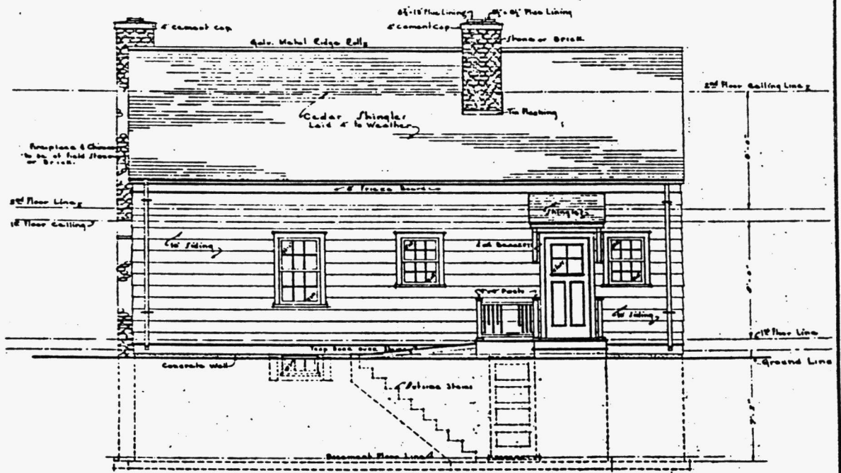
• REAR • ELEVATION •
