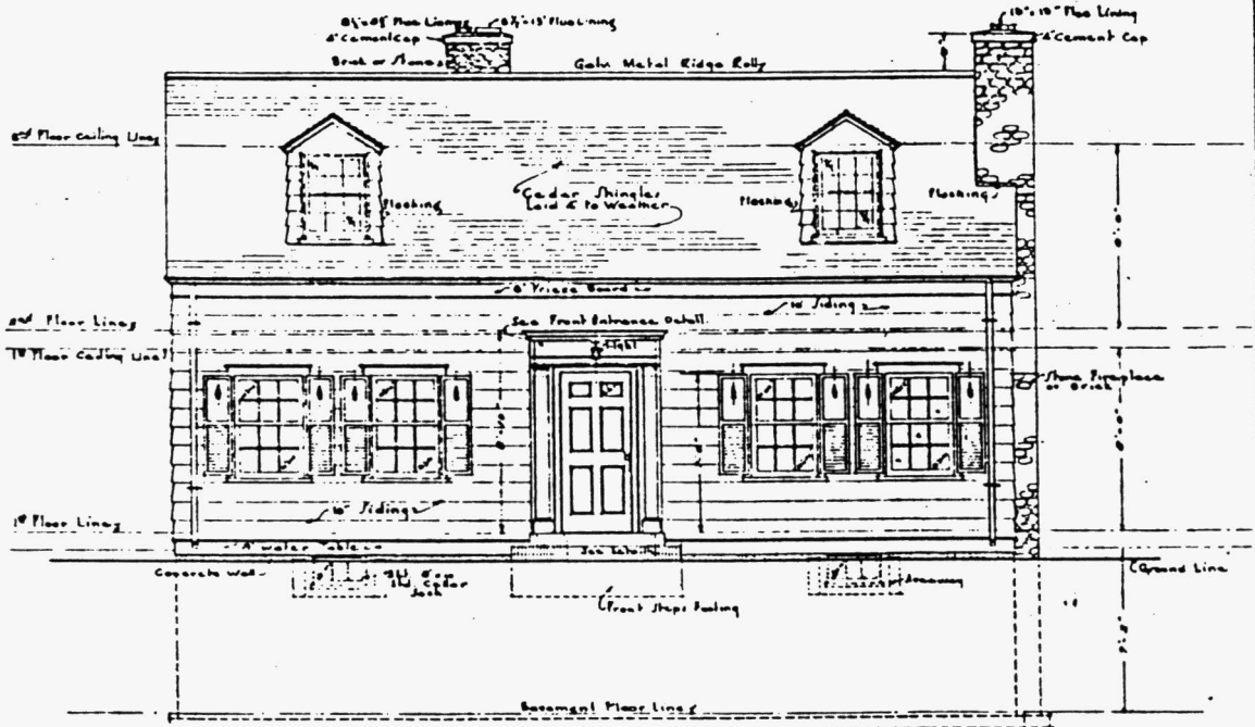
• FRONT • ELEVATION •
