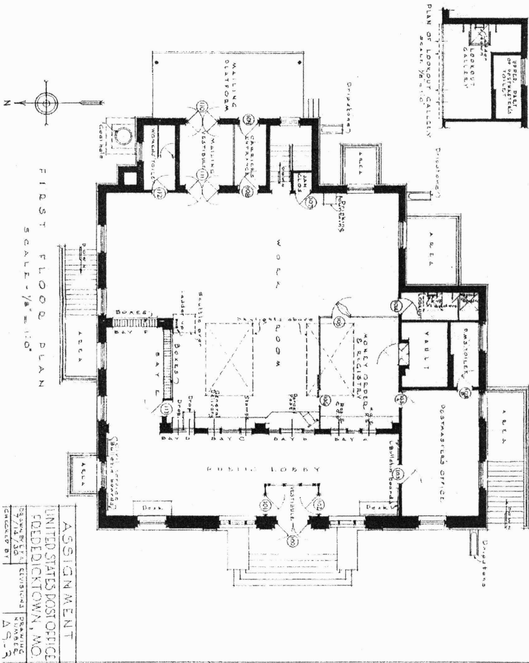
Figure 4: Original First Floor Plan
