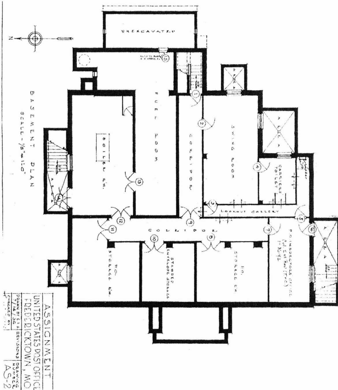
Figure 5: Original Basement Floor Plan
