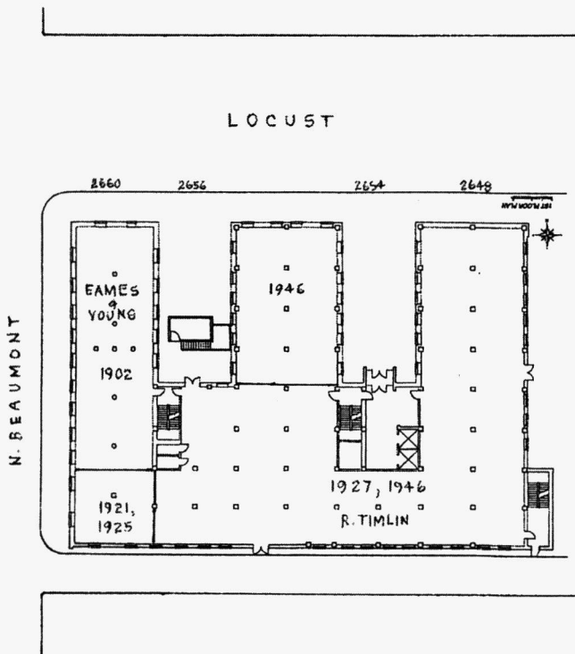
Figure 1: Beaumont Telephone Exchange Floorplan. June 2005. Courtesy of Garen Miller, A.I.A. Adapted by Landmarks Association of St. Louis.
