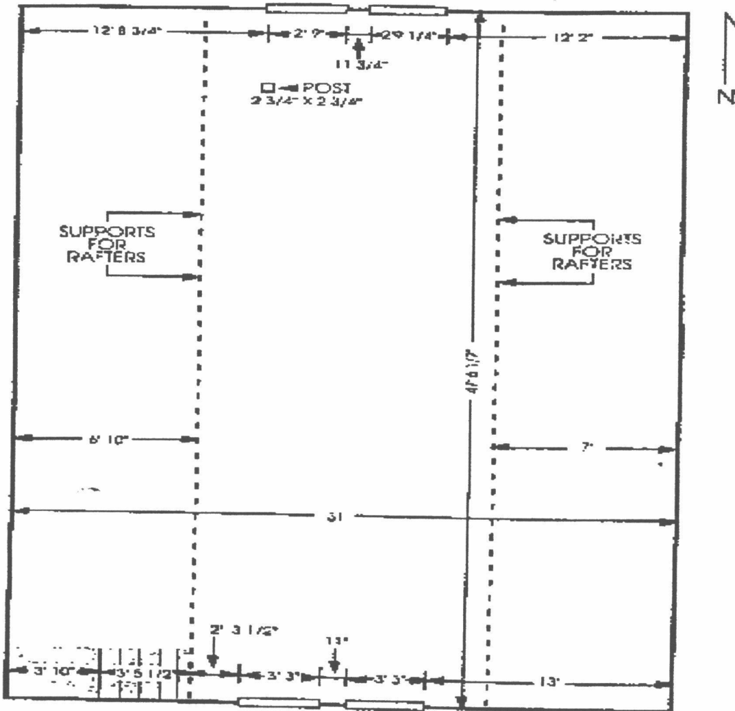
Third floor, Greer Mill.
